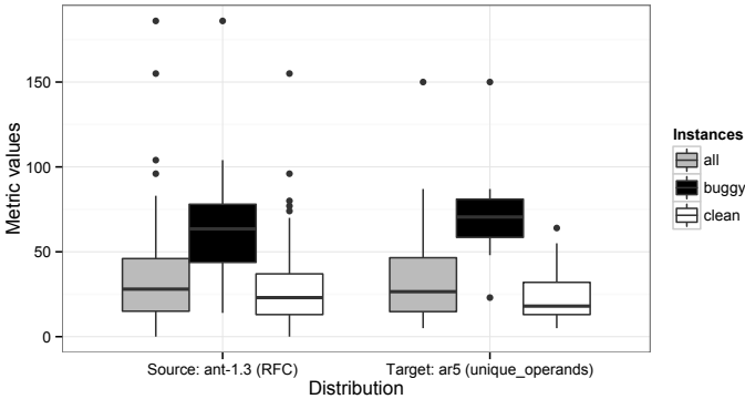
Fig. 4: Distribution of metrics (matching score=0.91) from ant-1.3 \Rightarrow ar5 (AUC=0.946).
