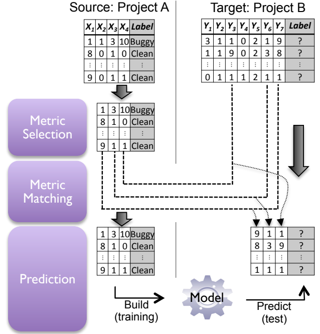
Fig. 2: Heterogeneous defect prediction
